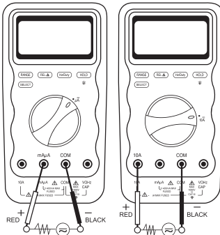
SERIES CONNECTION
